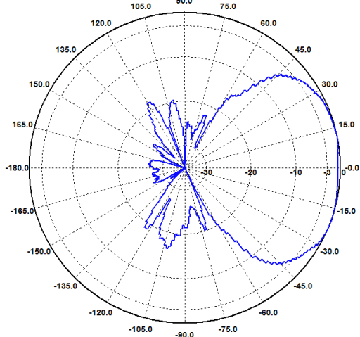
E-Ebene / E-Plane 3.5 GHz
