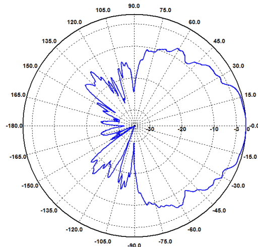
H-Ebene / H-Plane 8.0 GHz
