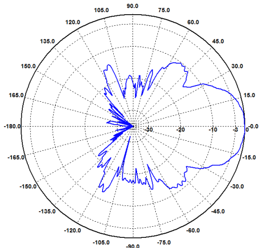
E-Ebene / E-Plane 8.0 GHz
